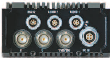
LinkXP, L1103, Bottom View
